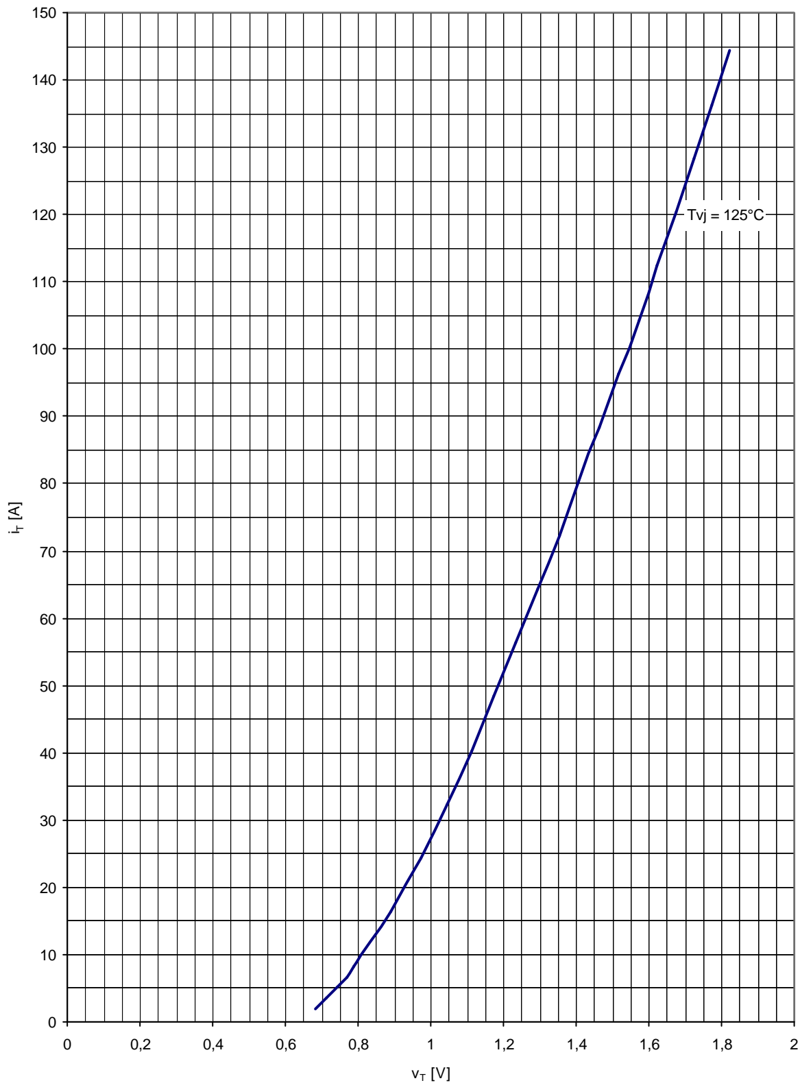
Grenzdurchlaßkennlinie / Limiting on-state characteristic i_T = f(v_T)
